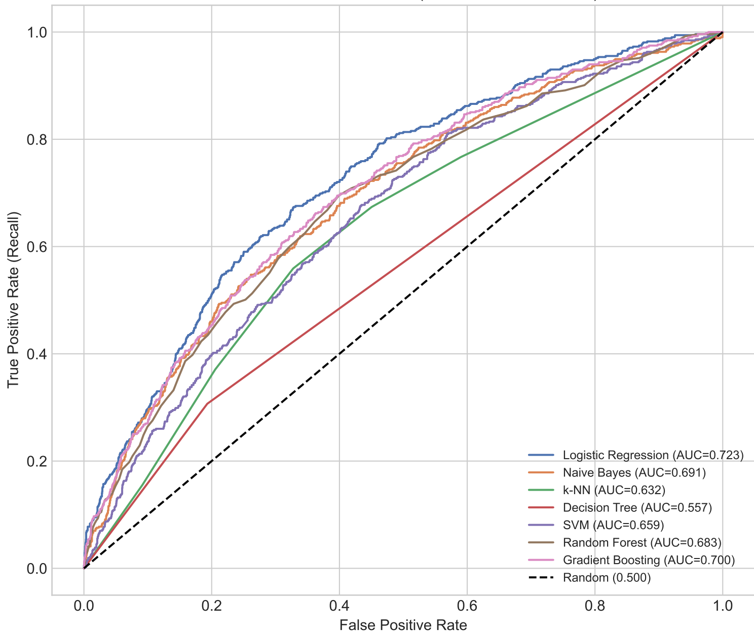
ROC curves — all models (5-fold cross-validated)
